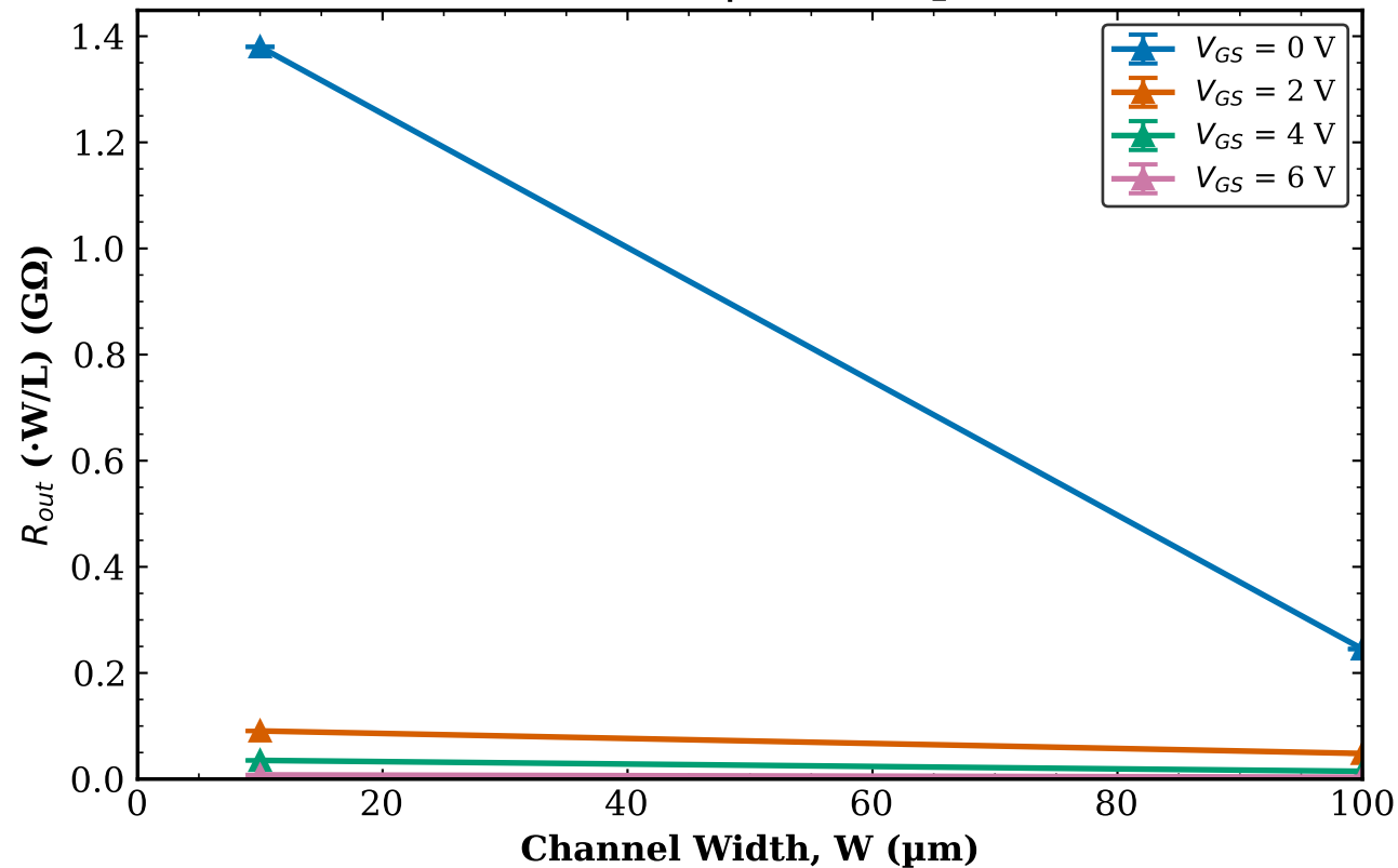
TFT3 Transistor 1 R_{out} vs W | L = 10\text{ }\mu\text{m}
